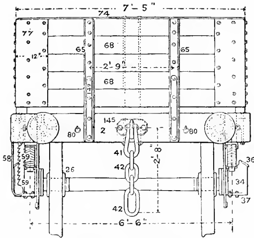
Fig. 350. End Elevation.
